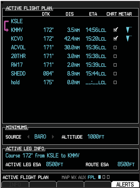
Active Flight Plan Page
