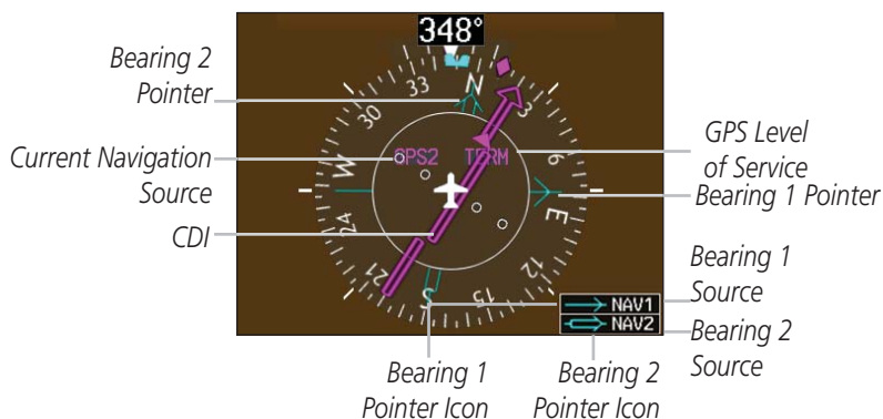
Bearing Pointers on the HSI
