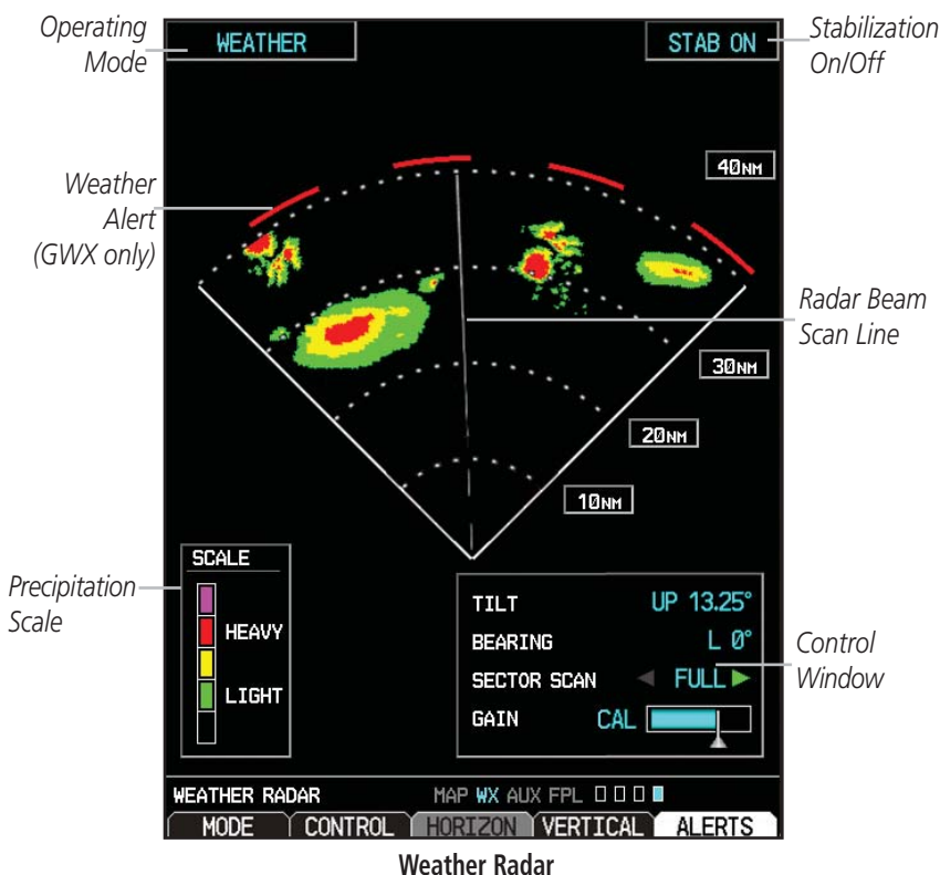
Weather Radar
